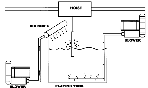
SOLUTIONS BLOW-BACK
